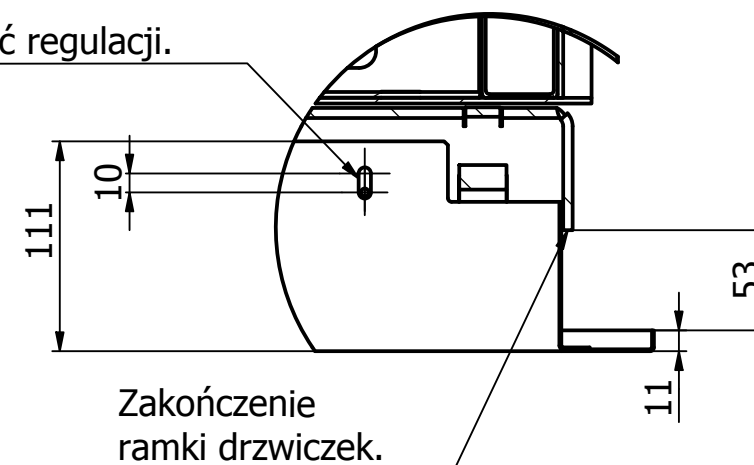
C (1:4)
