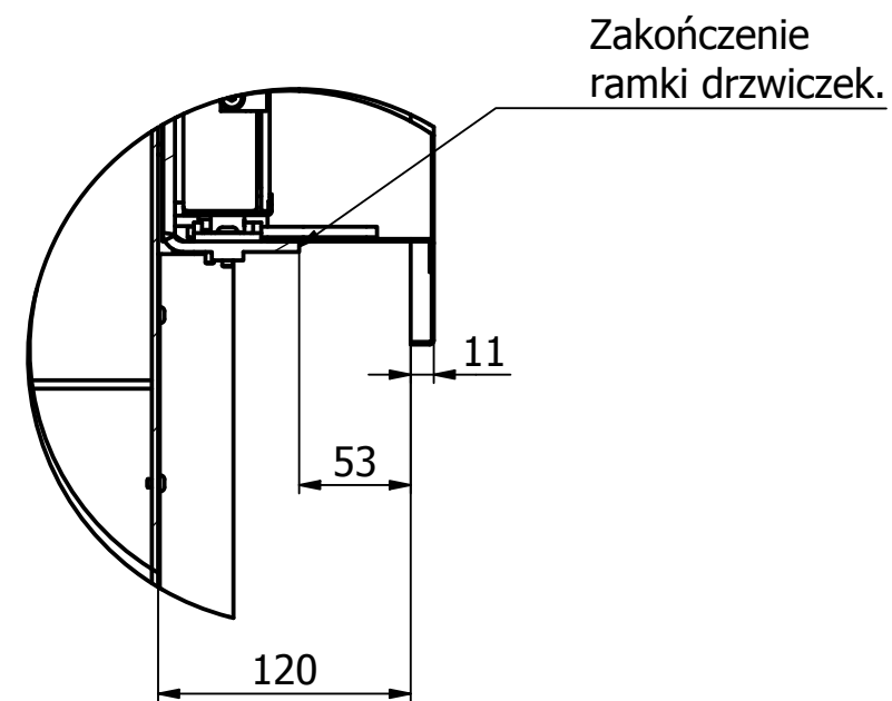
B (1:4)
