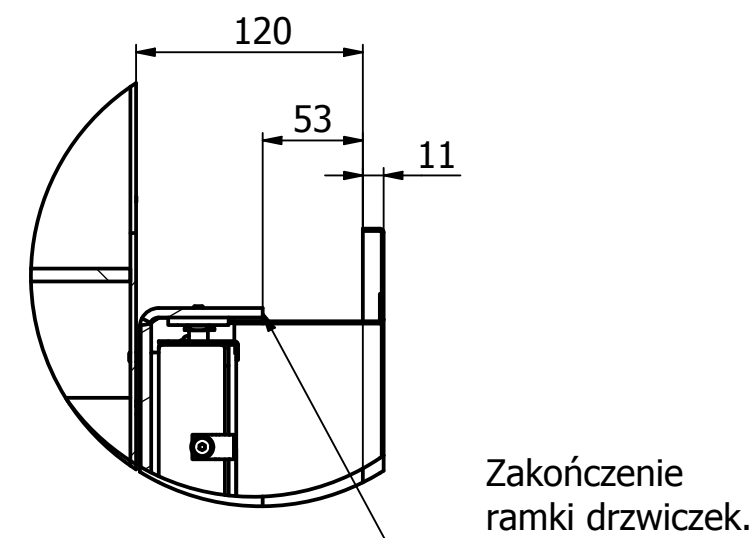
A (1:4)
