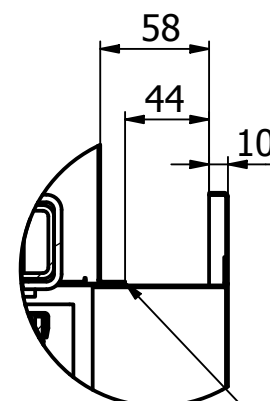
C (1:4)
